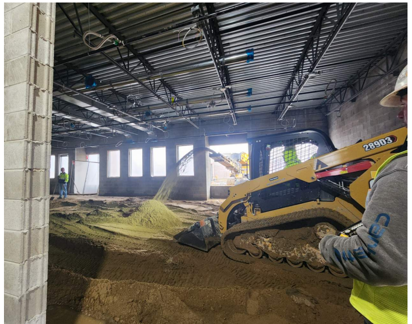
Sand being shot into the building and spread by a skid steer.
