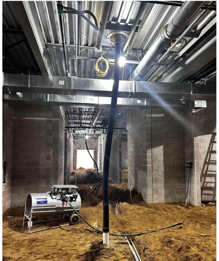
Roof drain connection to keep sand dry.
